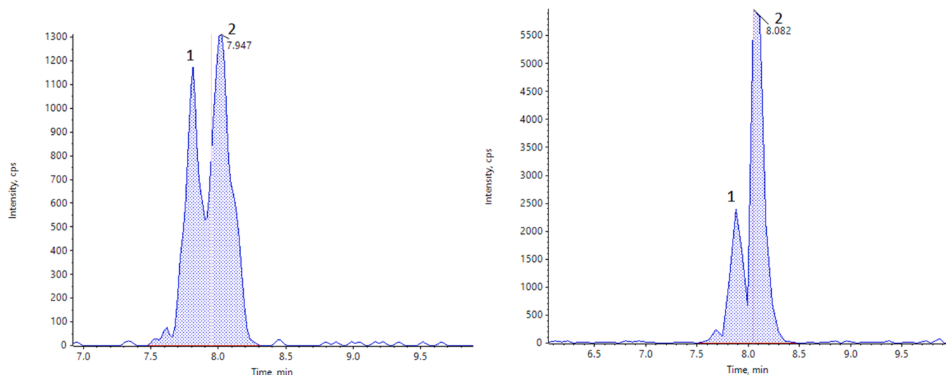
Fig. 3. Chromatograms of PFOS in insecticide 5 (right) and field 3 (left). The branched isomer of PFOS is labeled with 1 and the linear isomer of PFOS is labeled with 2.
